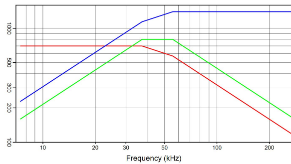
C-CAP 03 7 \mu\text{F} 700 V rms 1400 A rms 800 kVA r I(A) — Q(kVA r ) — V rms
