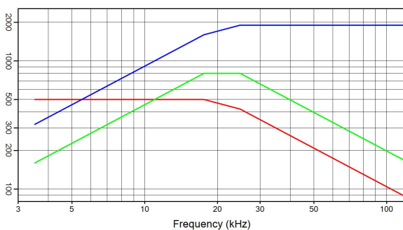
C-CAP 03 29 \mu\text{F} 500 V rms 1900 A rms 800 kVA r I(A) — Q(kVA r ) — V rms
