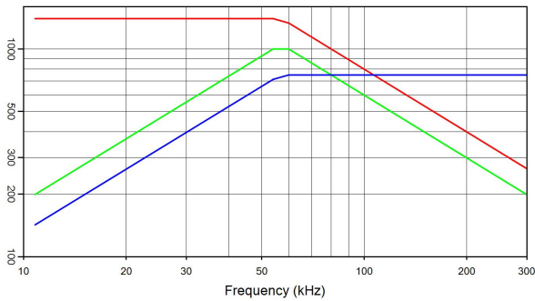
CMF 1.5 \mu\text{F} 1400 V rms 750 A rms 1000 kVA r I(A) — Q(kVA r ) — V rms —
