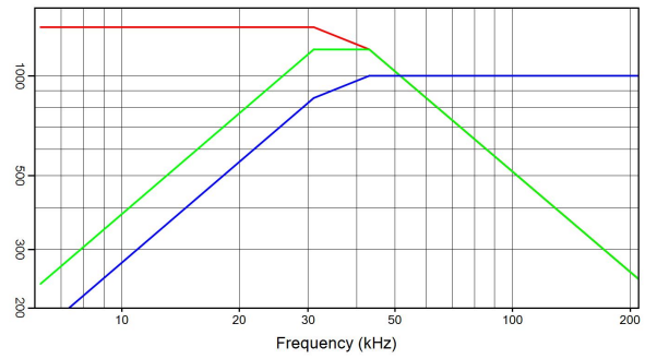
CMF 3.1 \mu\text{F} 1400 V rms 1000 A rms 1200 kVA r I(A) — Q(kVA r ) — V rms —
